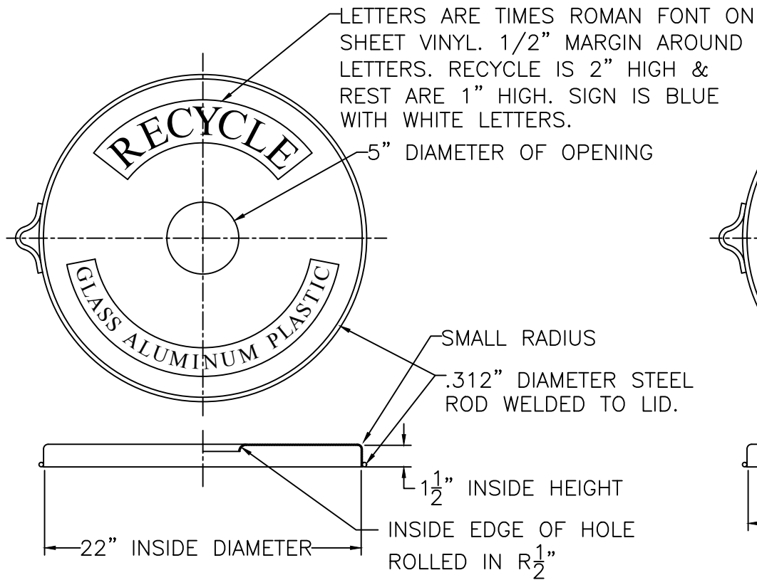
RECYCLE LID WITH \phi 5" HOLE
